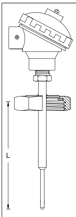
BSM PROCESS CONNECTION HYGIENIC WELDS REDUCED TIP
