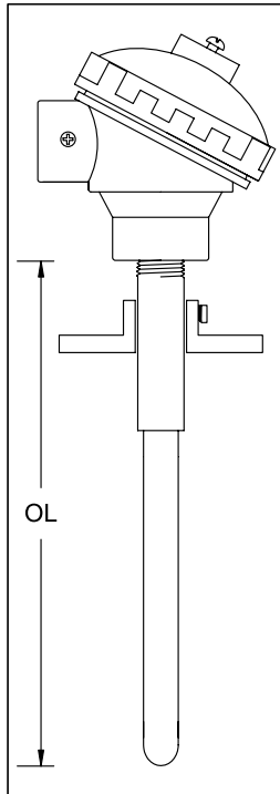
HIGH TEMPERATURE THERMOCOUPLE C/W ADJUSTABLE FLANGE
