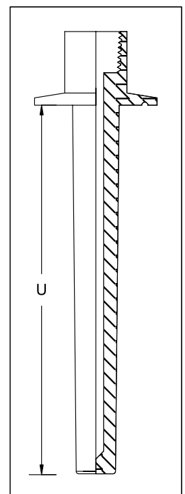
316SS THERMOWELL WITH TRICLOVER FLANGE
