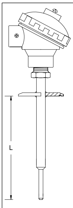
TRICLOVER PROCESS CONNECTION HYGIENIC WELDS REDUCED TIP
