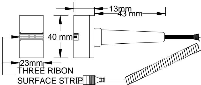
MAGNETIC SURFACE MODEL TCLM3R
