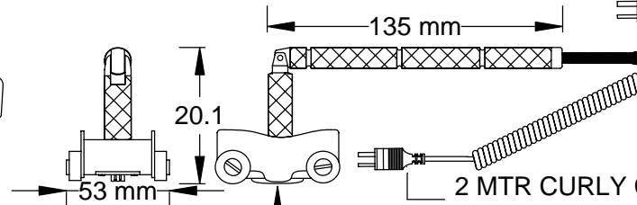
ROLLER CONTACT MODEL TCKROLLER
