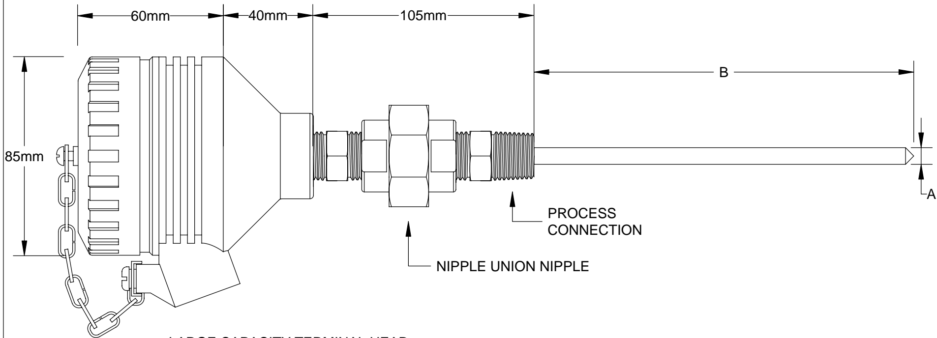
LARGE CAPACITY TERMINAL HEAD INTERNAL - 62mm Ø x 36mm HIGH Suitable for 33mm and 40mm centres
