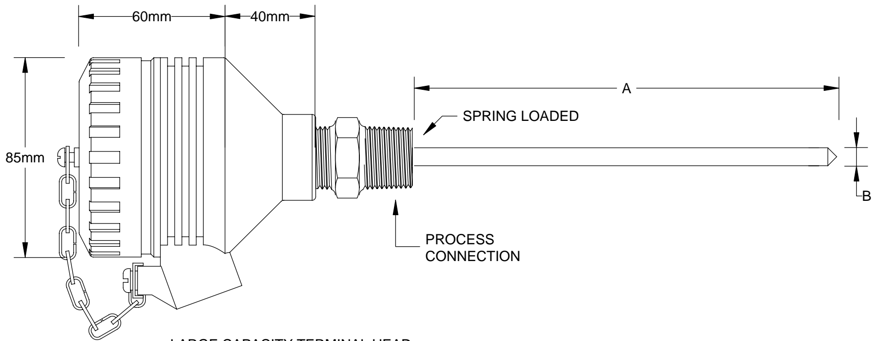
LARGE CAPACITY TERMINAL HEAD INTERNAL - 62mm Ø x 36mm HIGH Suitable for 33mm and 44mm centres
