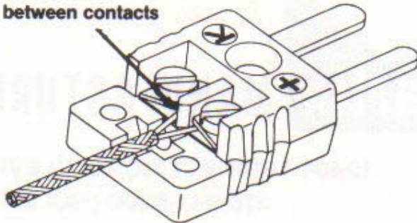
Wire Jab-In ® between contacts
