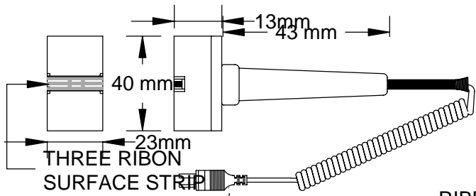
MAGNETIC SURFACE MODEL TCLM3R
